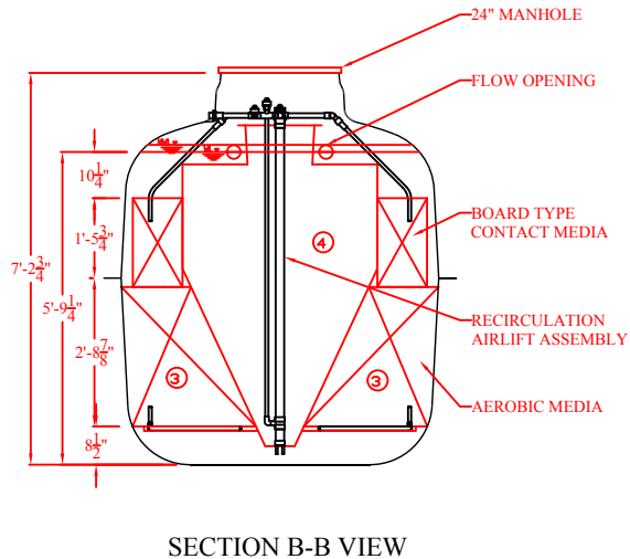
SECTION B-B VIEW
