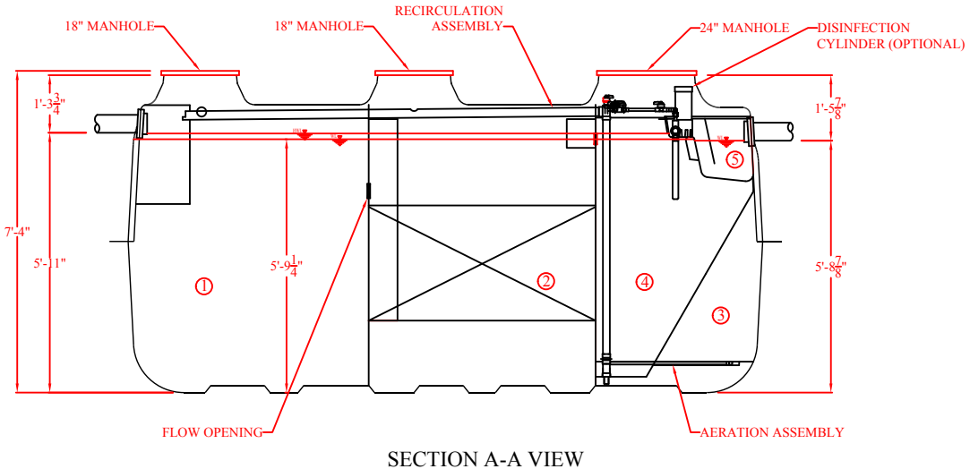
SECTION A-A VIEW
